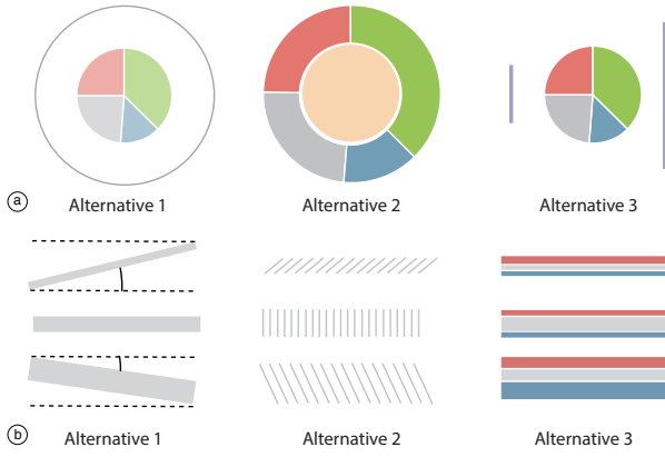
Fig. 5. Design alternatives of a) the default snapshot glyph and b) the transition glyph. For the transition glyphs, three different types of tie strength changes are indicated: increasing, constant, and decreasing (from top to bottom).
