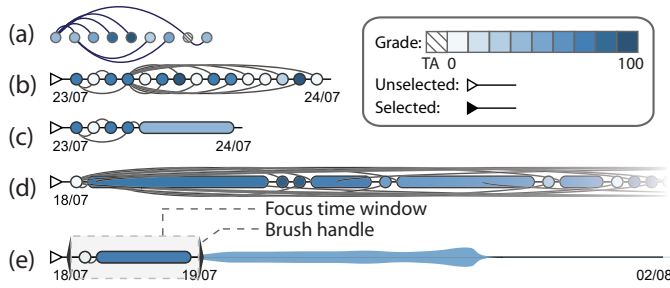
Fig. 5. The design process of Thread River. (a) The basic Thread Arcs. (b) Thread Arcs not scaling well for a number of posts. (c) The revised Thread Arcs with aggregation in subsequent posts replying to the same post, showing the same thread as that in (b). (d) The design of revised Thread Arcs showing lengthy thread with complex reply relationships, which is too long to display. (e) The Thread River design presenting the same thread as that in (d).
