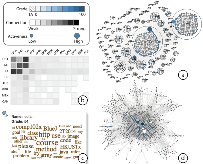
Fig. 6. (a) The grouped node-link diagram. (b) The heatmap matrix showing group level connections. (c) Informative tooltip pops out when a user hovers over a node. (d) The basic node-link diagram based on MDS and force directed layout.
