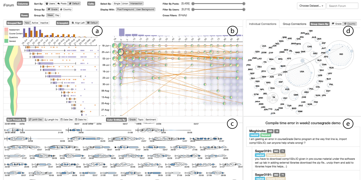
Fig. 1. Using iForum to explore the MOOC forum of a JAVA programming course that has attracted more than ten thousand students during a ten-week course period. (a) The Overview shows the overall changes of posts, threads, and users on the forum. (b) The Matrix View further enables the comparison of dynamic patterns of different user groups along time. After a cell of interest is selected, orange lines are shown on top of the matrix to indicate the threads passing through that cell. (c) Meanwhile, the Thread View presents all selected threads in a compact layout, and (d) the Social Network View reveals the interactions among corresponding users based on their replying relationships. (e) When a specific thread is selected, the Text View displays discussions in traditional indented form.
