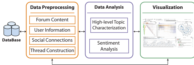
Fig. 2. Overview of the iForum system architecture.
