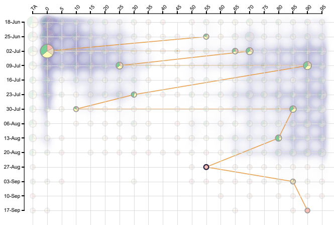
Fig. 8. An orange line passes through multiple pie charts starting from the second row till the last row in the matrix diagram, showing that the thread was active across a long time period. In addition, these pie charts locate in different columns, indicating users with different performance were involved into the thread.
