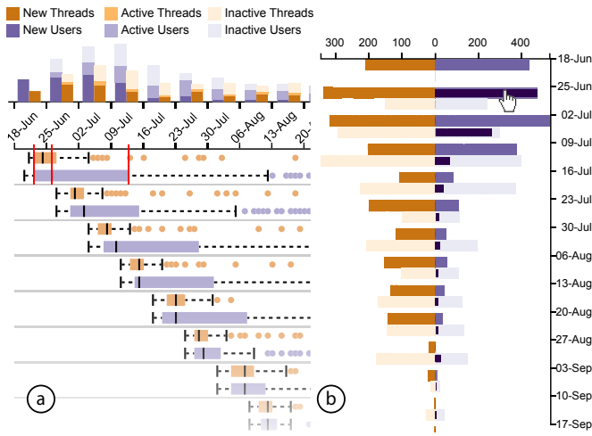
Fig. 3. The comparison between (a) the G-boxplot and (b) the grouped bar charts.
